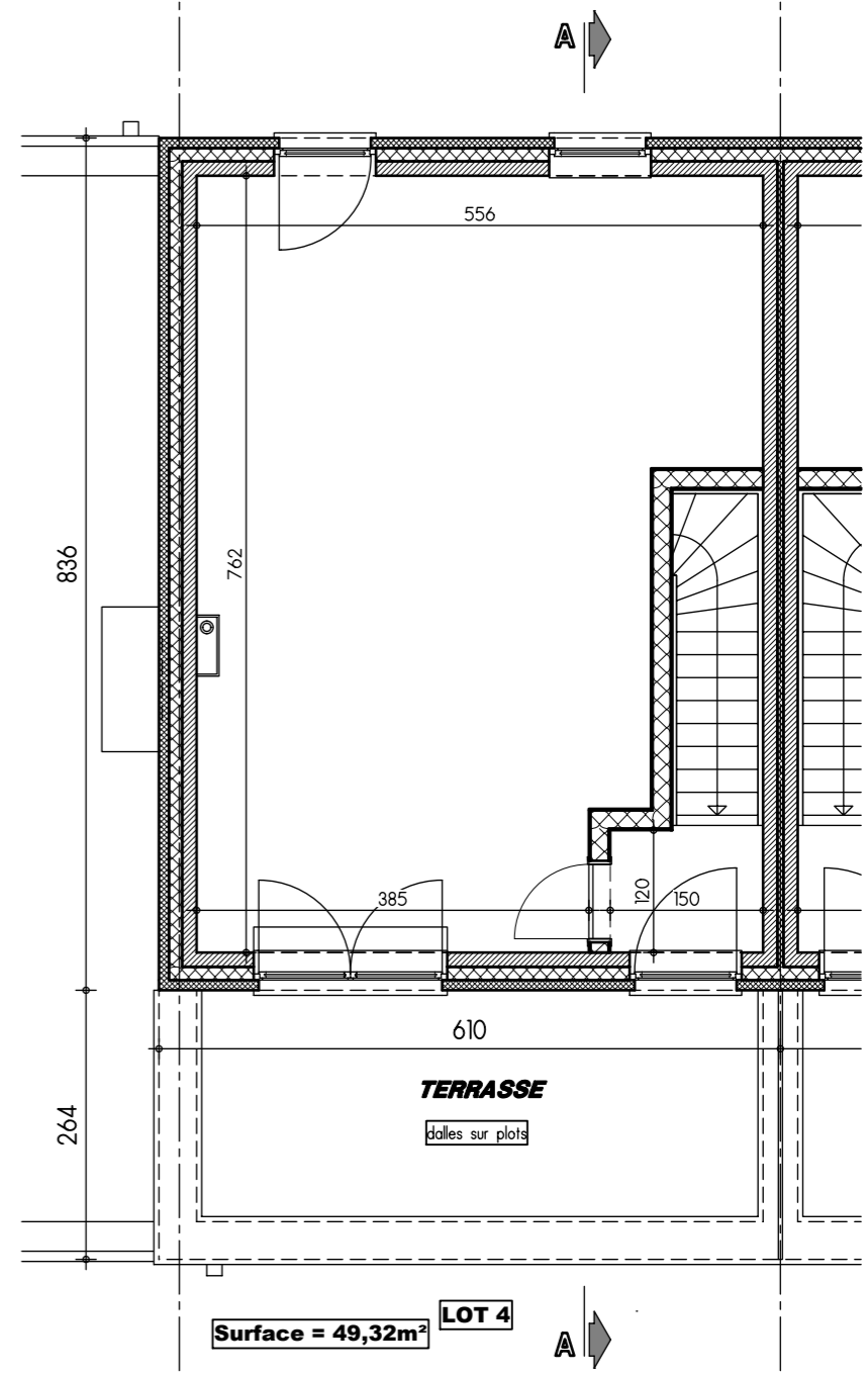
PLAN COMBLES
